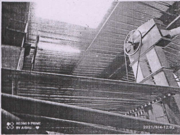
Pitting into Roller Dehusker
